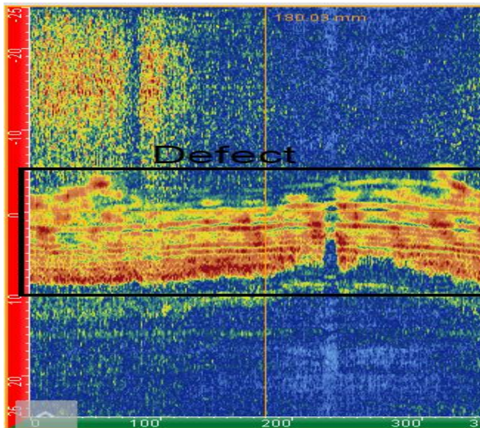
Inspection C-scan image showing the chevron crack across 360 degrees in a cylindrical shaft
