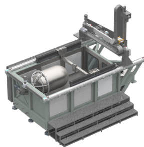
Propellant Tank Inspection Immersion Ultrasonic System
